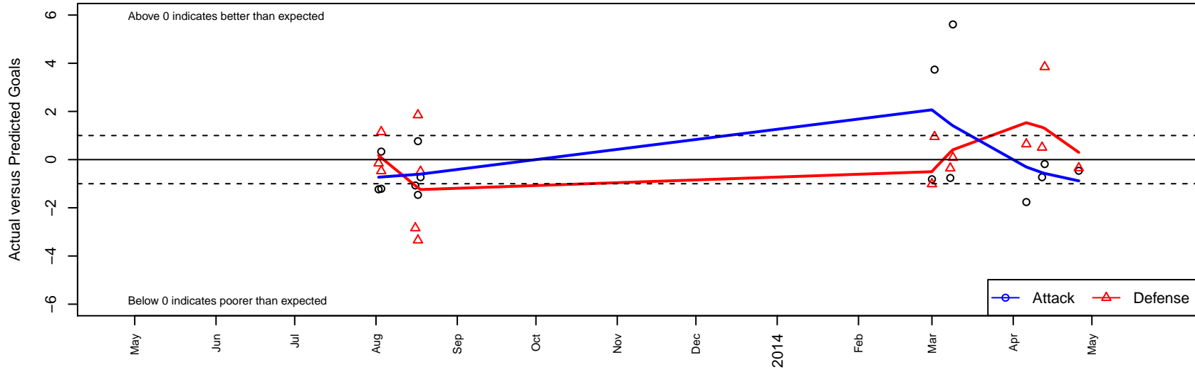
Bend FC Timbers White G02 Dots are actual minus expected GF (blue circles) and GA (red triangles). Blue line is smoothed change in attack strength. Red is smoothed change in defense strength.
